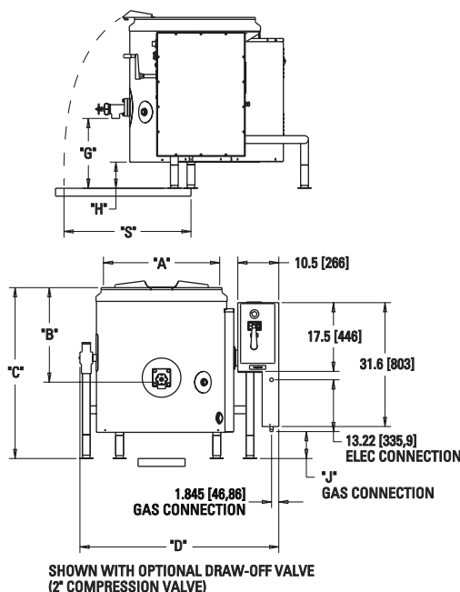
SHOWN WITH OPTIONAL DRAW-OFF VALVE (2" PLUG VALVE)
